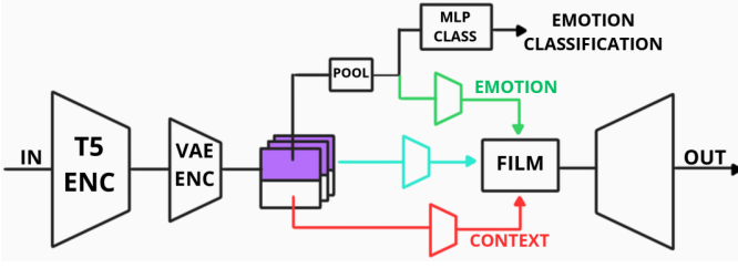
Figure 4: 5 → split-FiLM VAE Decoder.
